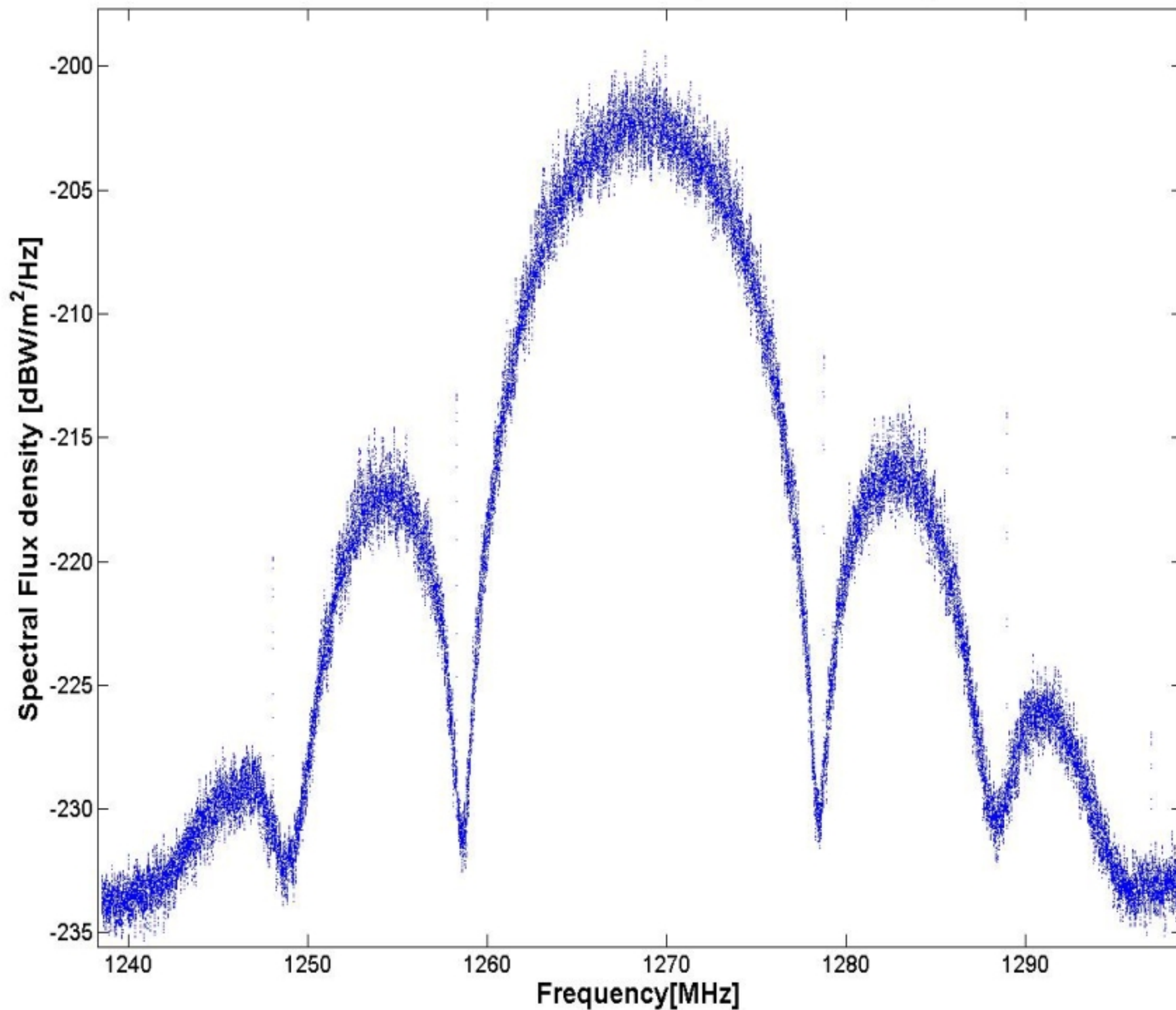
COMPASS/Beidou G3 - B3 Spectral Flux Density
