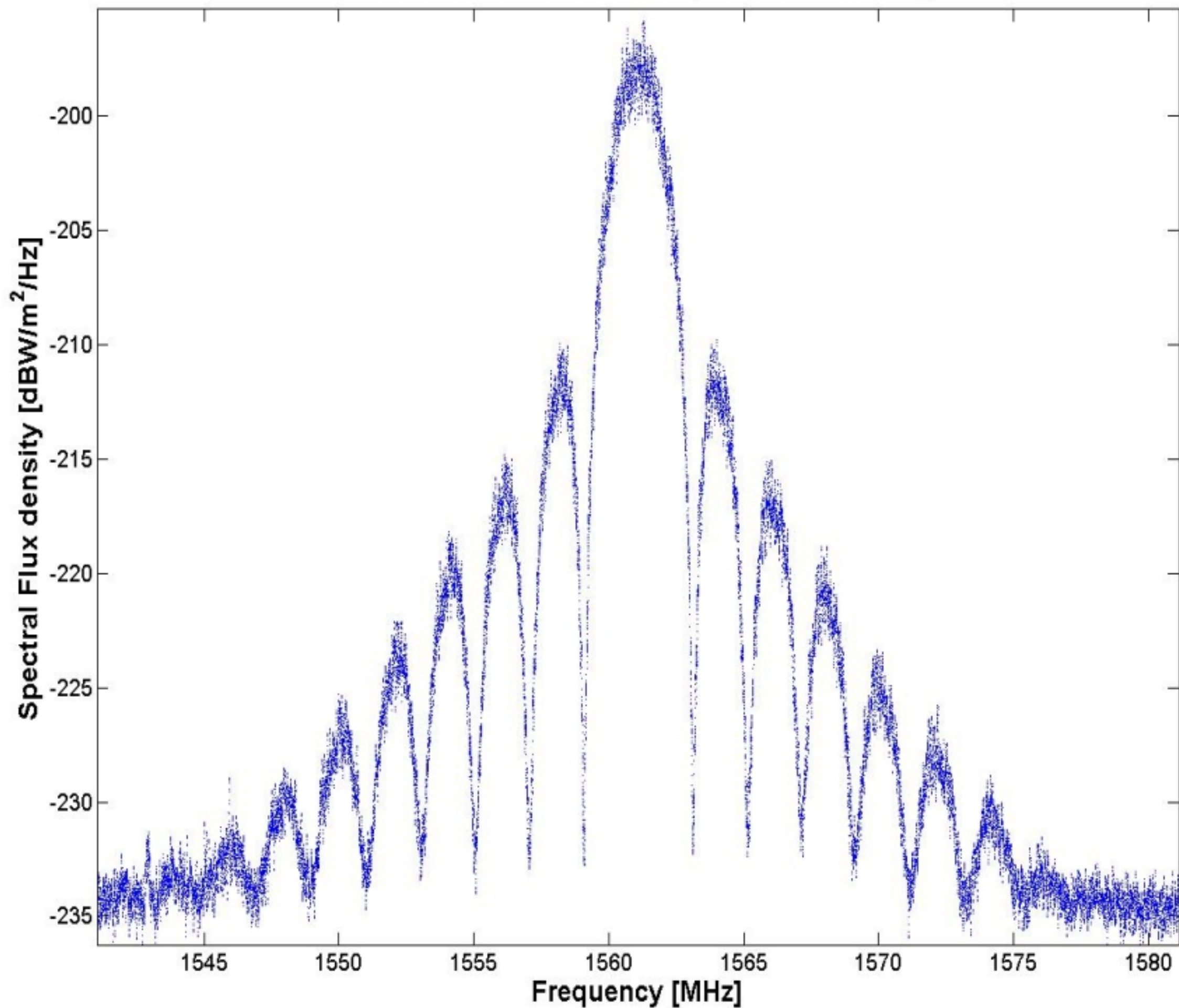
COMPASS/Beidou G3 - B1 Spectral Flux Density
